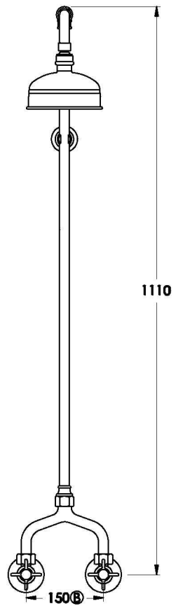
Front view
