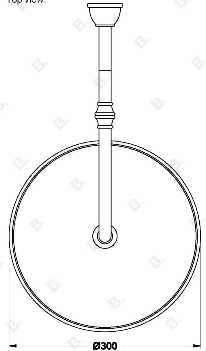
Top view:
