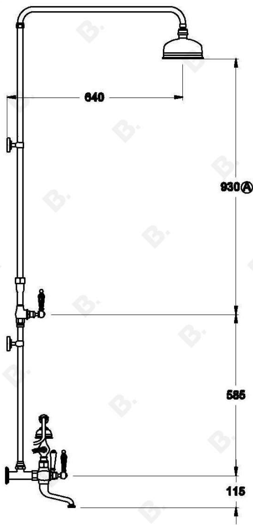
Side view:
